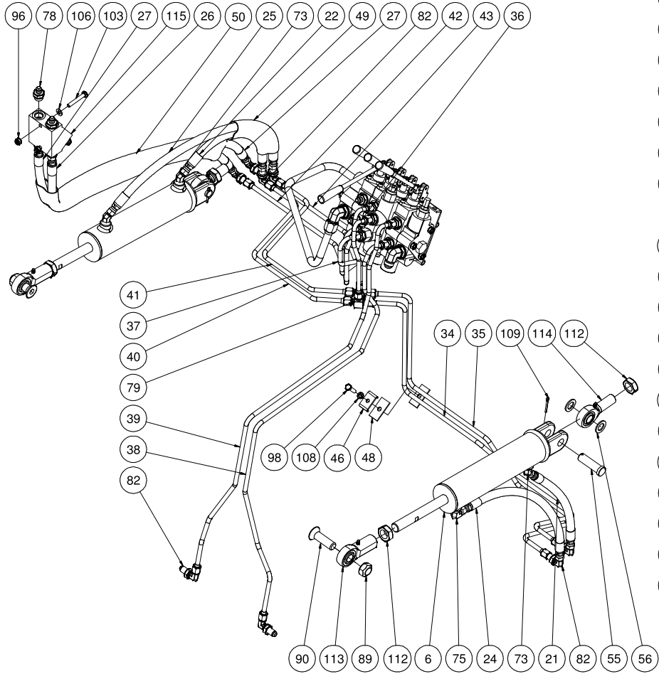
Mast Tilt, Lift, and Retractable Forks
