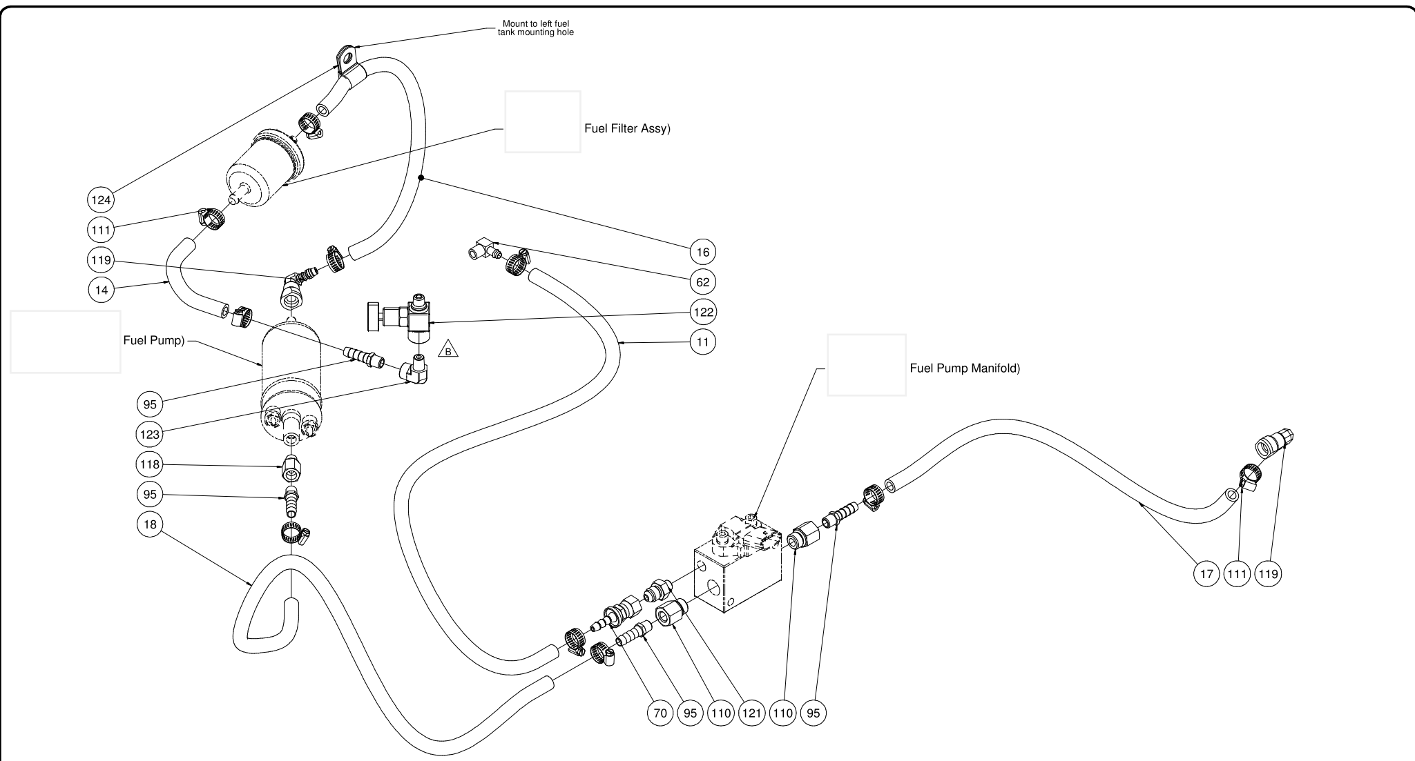
Gas Fuel System
